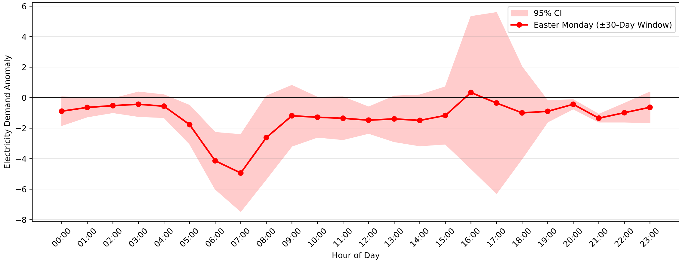
Dee Why West Demand Anomaly: Easter Monday (2008–2009, \pm 30 -Day Window)
